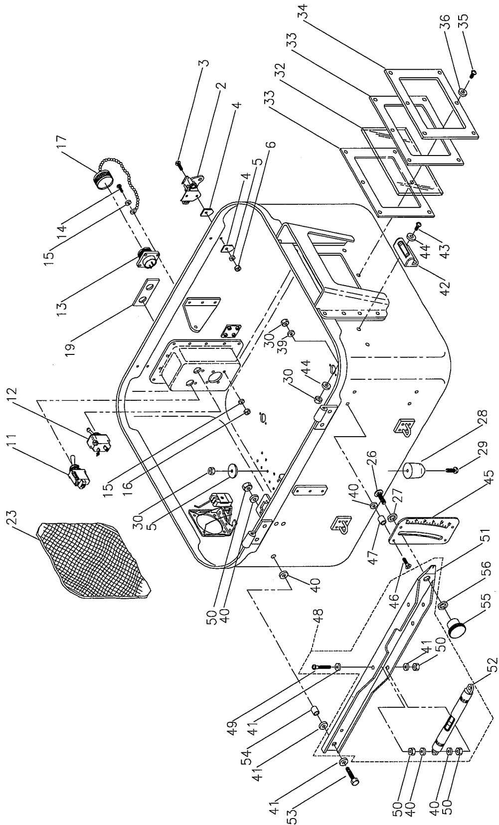
IPL Figure 3 Lower Housing Assembly
