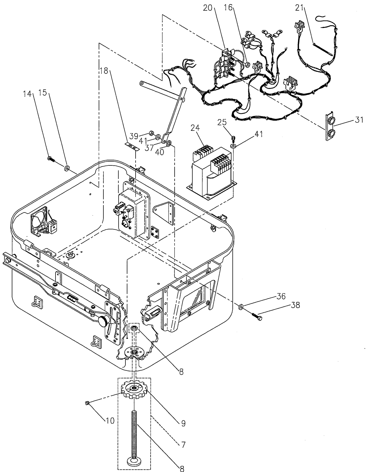
IPL Figure 3.1 Lower Housing Assembly
